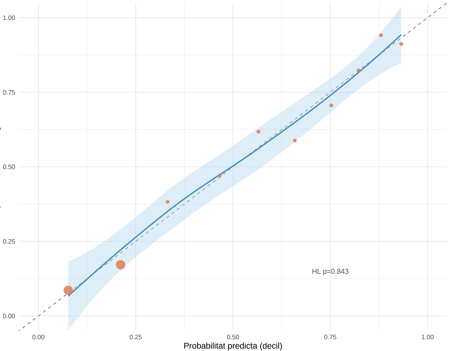
Calibration plot – Model logistic final (totes les dades)
